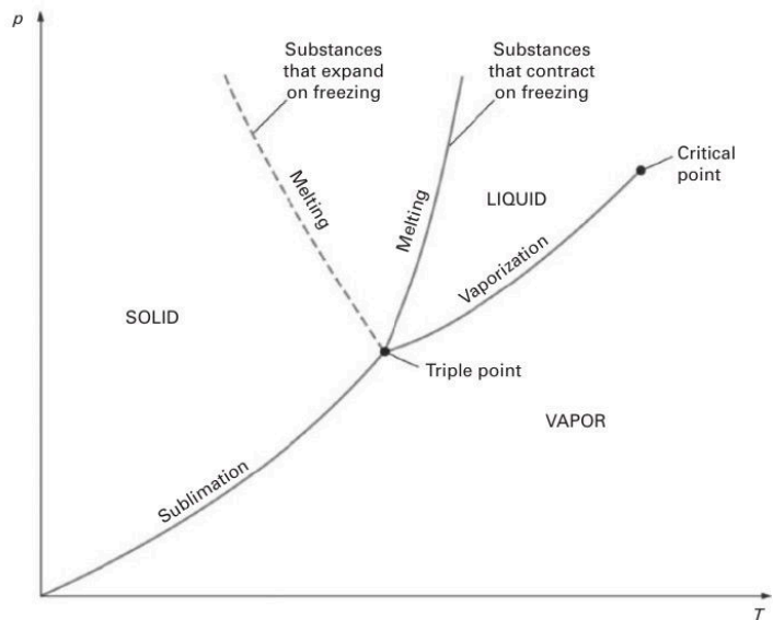
Figure 11.6 Phase diagram for simple compressible substance.
