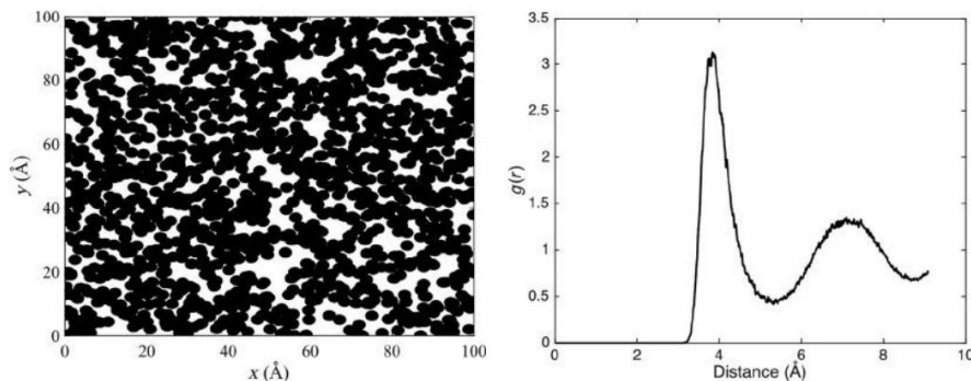
Figure 9.2 Radial distribution function for liquids.
