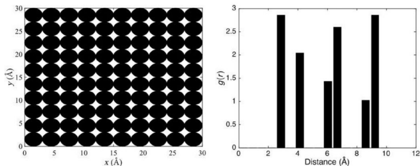
Figure 9.1 Radial distribution function for crystal structures.
