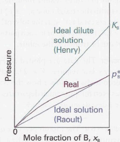
Fig. 5.15 When a component (the solvent) is nearly pure, it has a vapour pressure that is proportional to mole fraction with a slope p_B^* (Raoult's law). When it is the minor component (the solute) its vapour pressure is still proportional to the mole fraction, but the constant of proportionality is now K_B (Henry's law).
